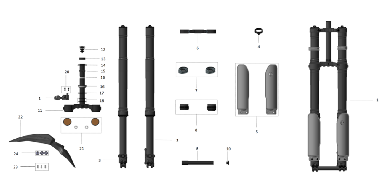
FIGURE-8 (Fr. Fork Assy.)
