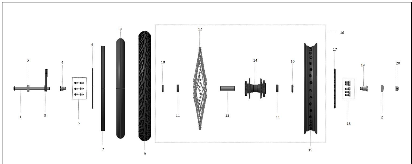
FIGURE-14 (Rr. Wheel Assy.)
