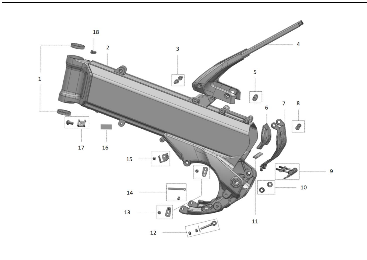
FIGURE-01 (FRAME)
