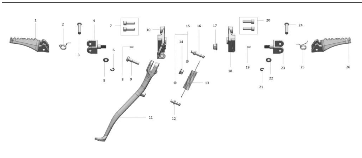
FIGURE-04 (Footpeg Assy.)
