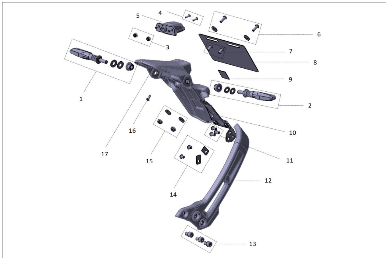
FIGURE-15 (License Plate Holder Assy.)
