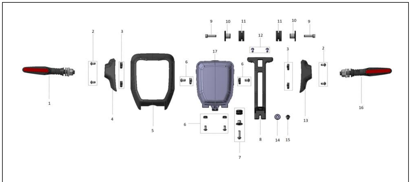
FIGURE-05 (Headlight Assy.)
