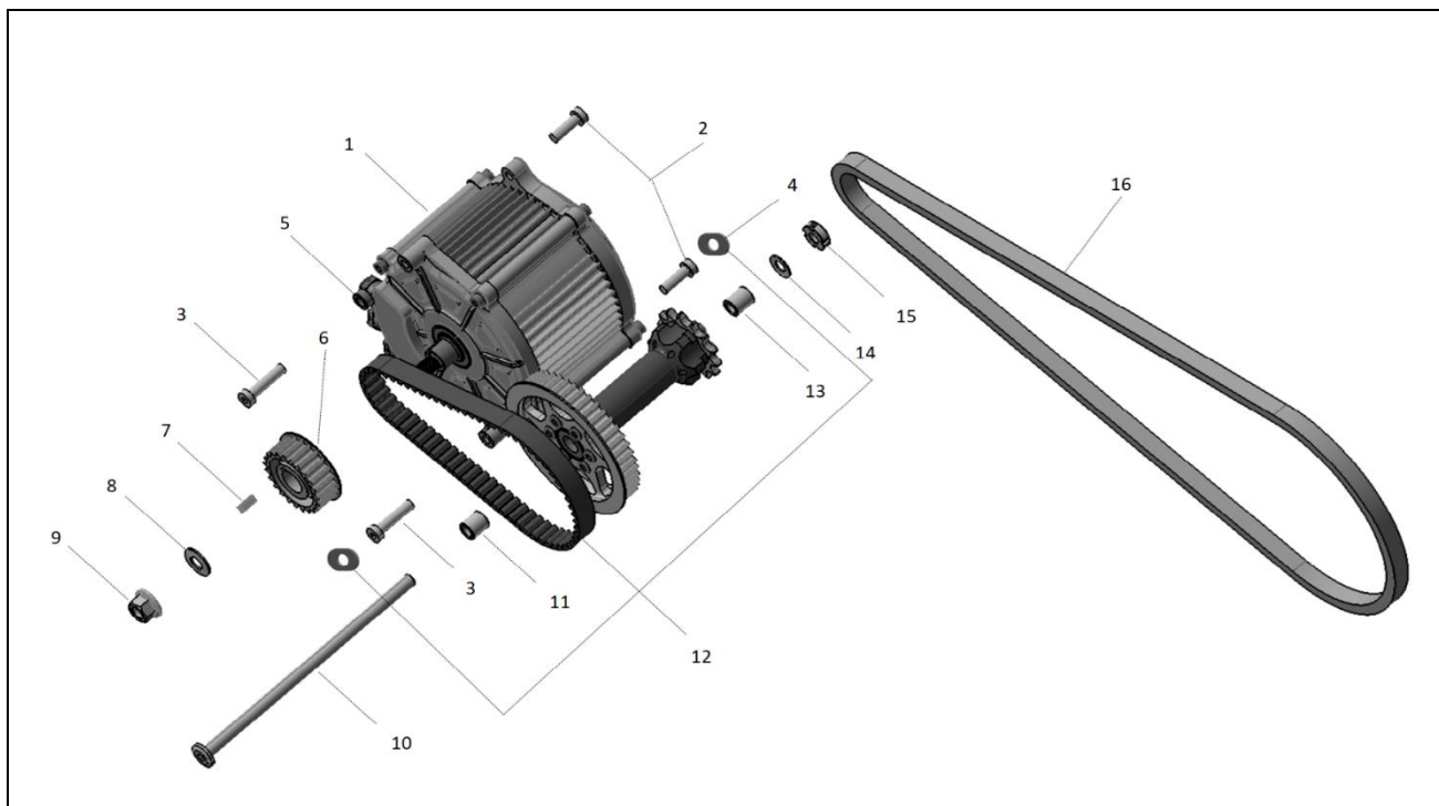
FIGURE-12 (Transmission Assy.)
