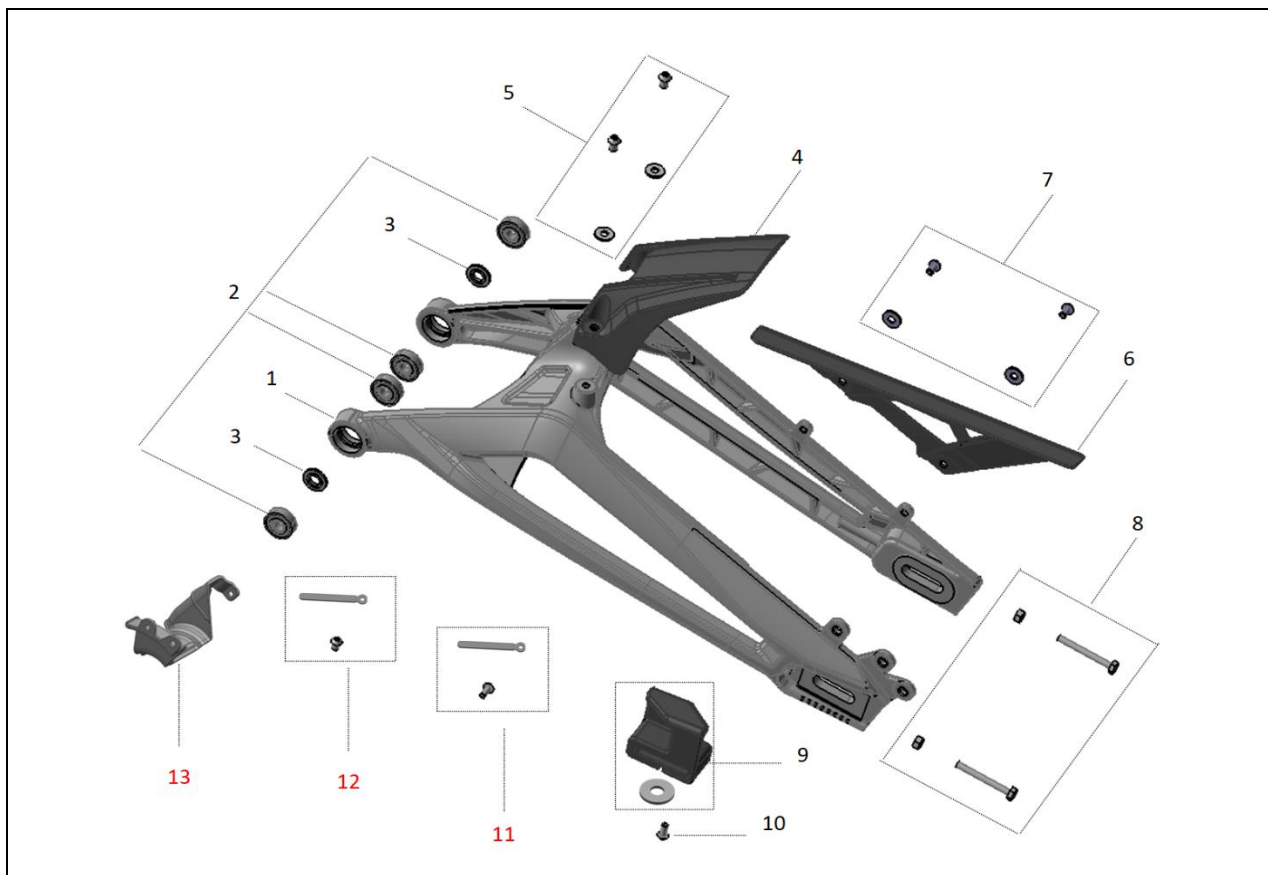
FIGURE-13 (Rr. Fork Assy.)
