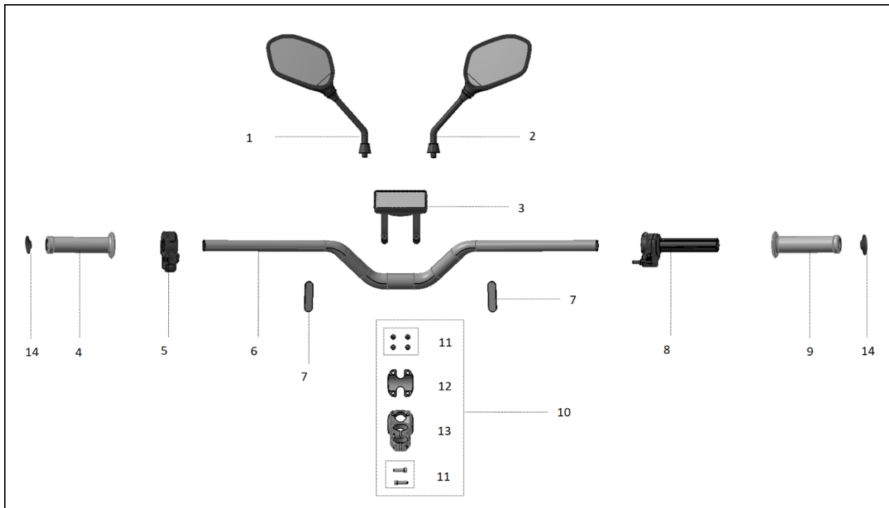
FIGURE-06 (Handlebar Assy.)
