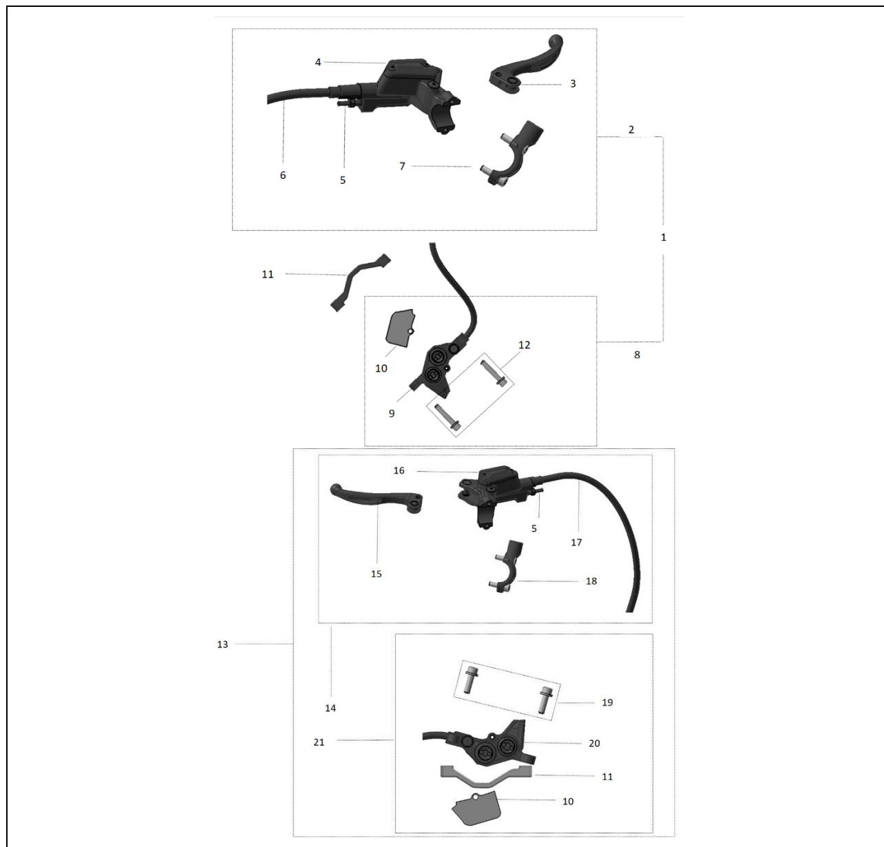
FIGURE-07 (Brake Assy.)
