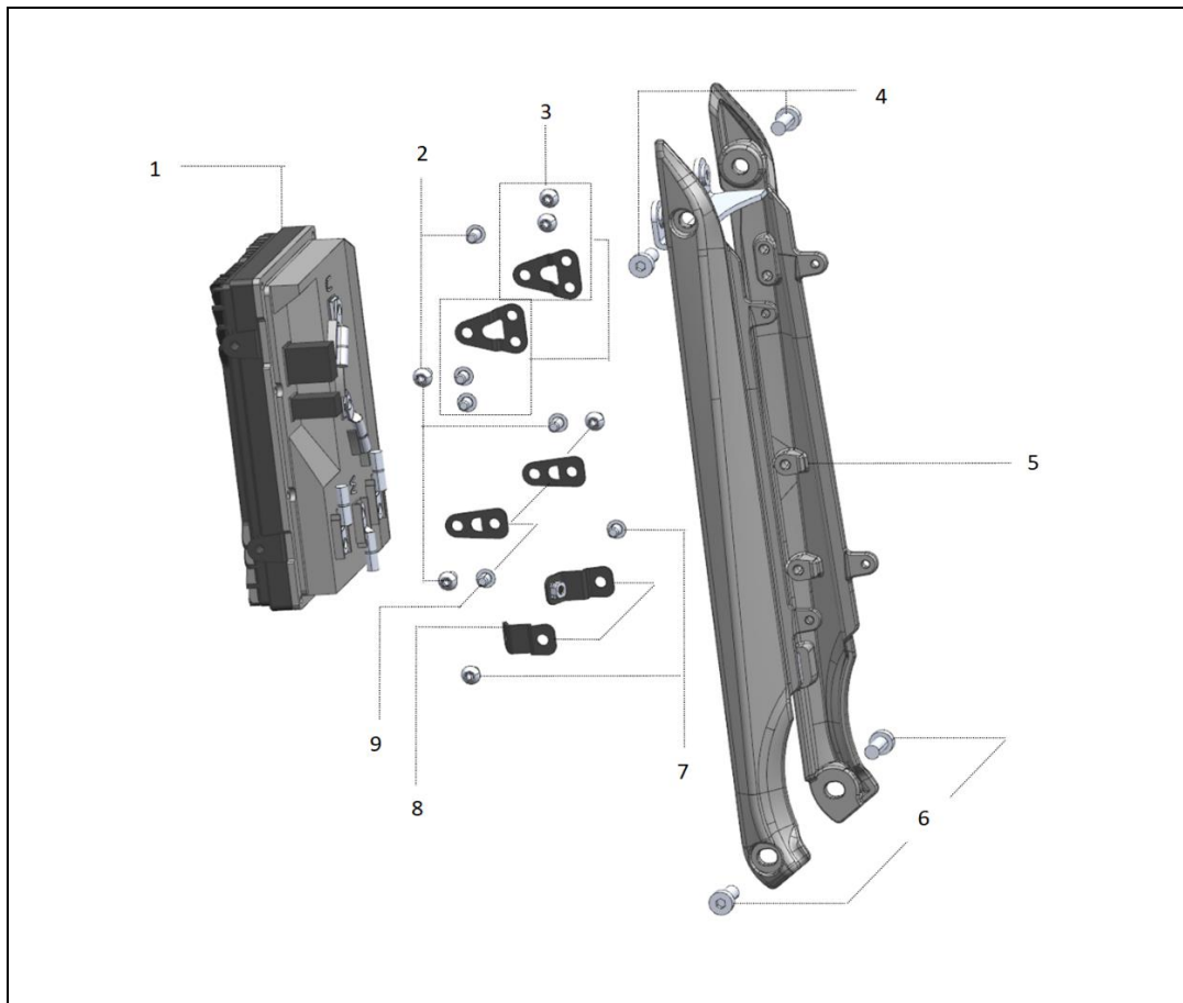
FIGURE-02 (Controller &amp; fr. Sub-Frame)
