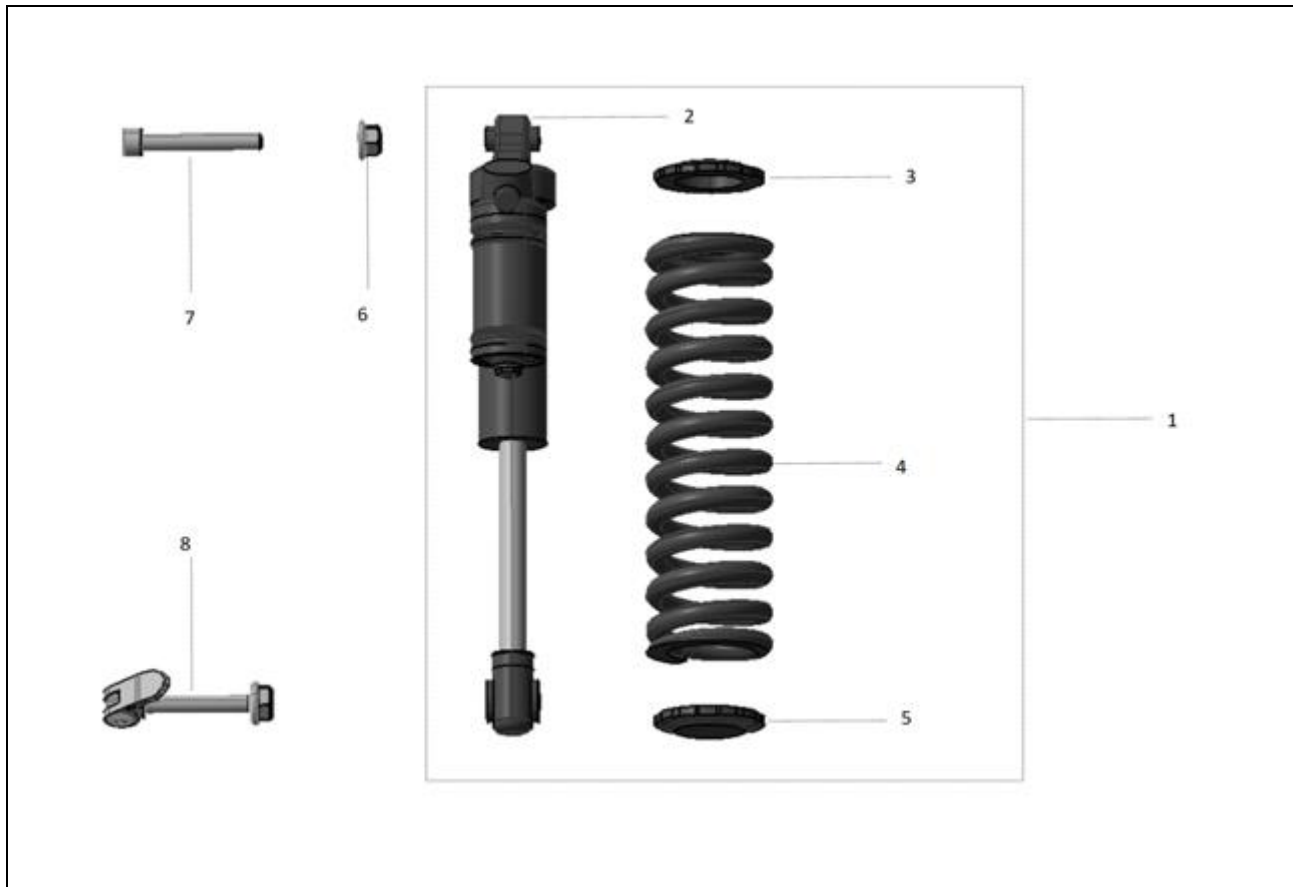
FIGURE-11 (Rr. Shock Absorber Assy.)
