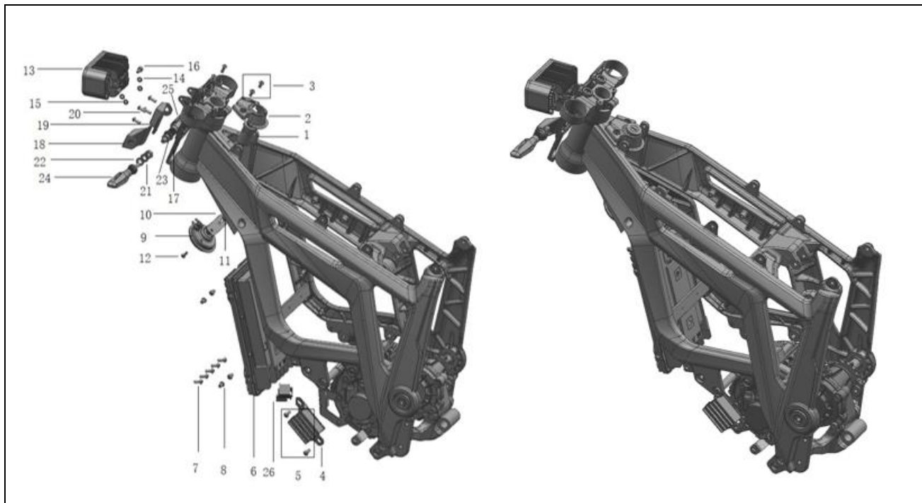
FIGURE-8 (ELECTRICAL PARTS)
