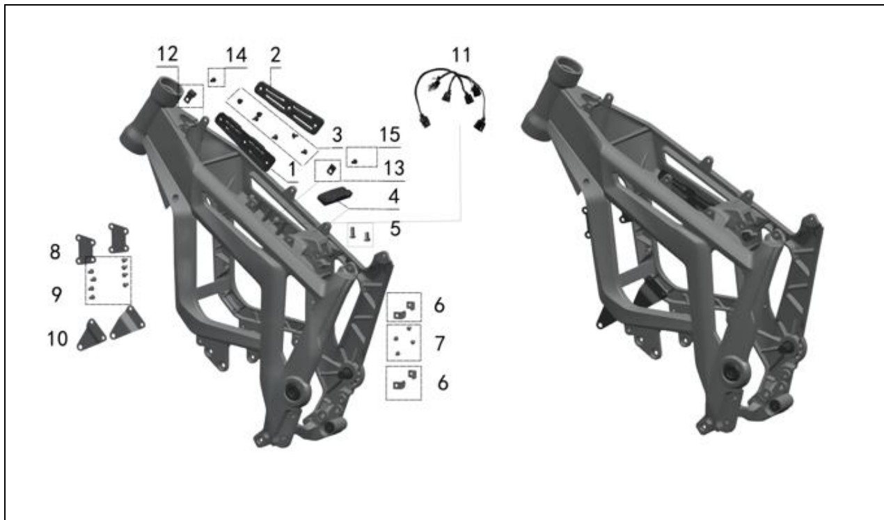
FIGURE-06(FRAME ASSY.)
