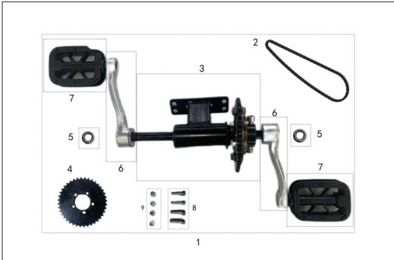
FIGURE-22 (Pedal Kit)
