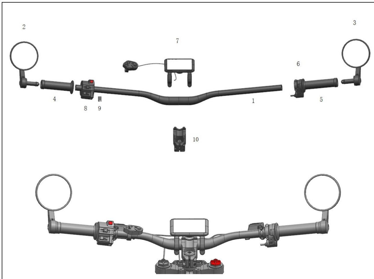
FIGURE-11 (Handlebar Assy.)
