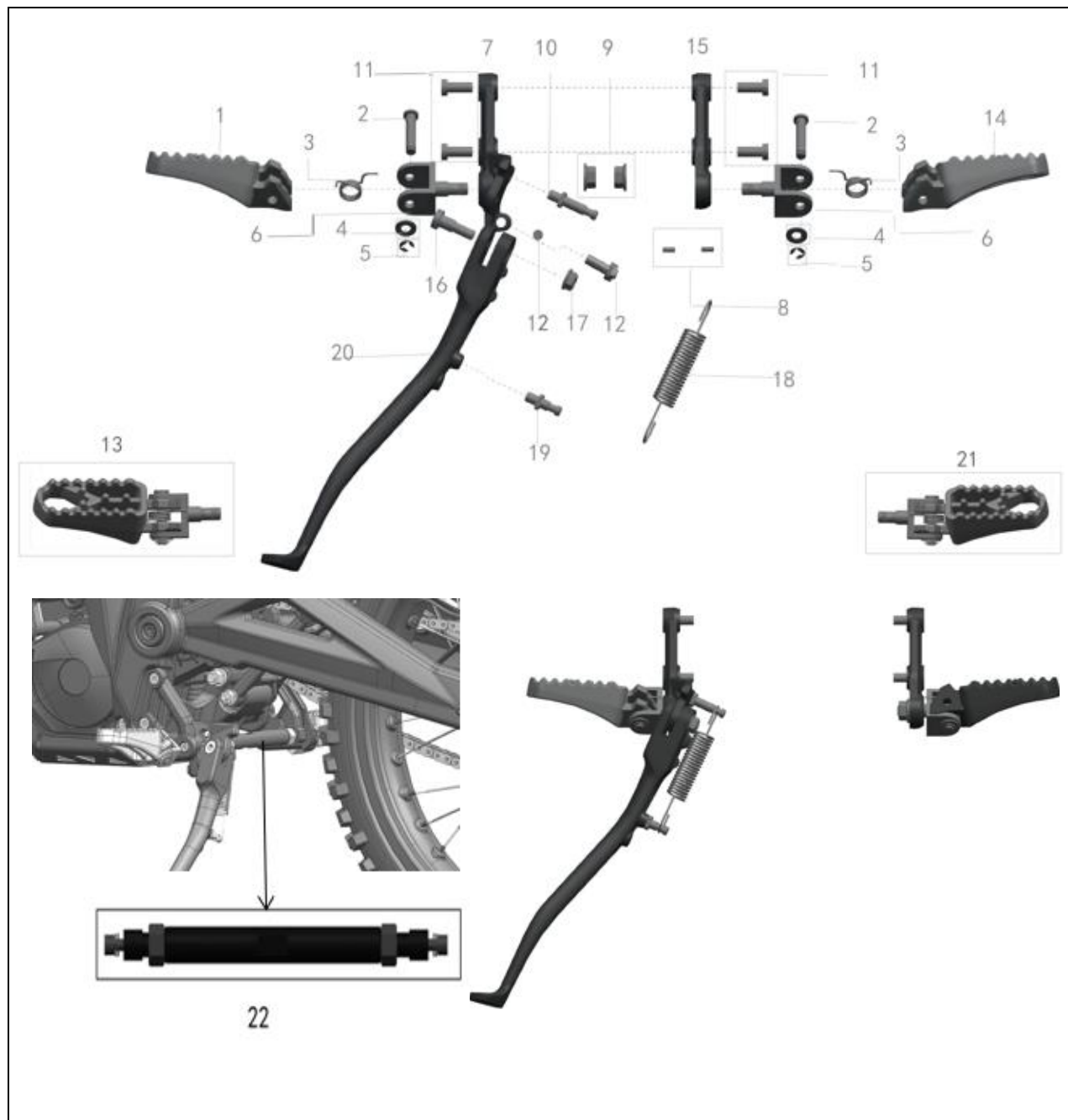
FIGURE-19 (Footpeg Assy.)
