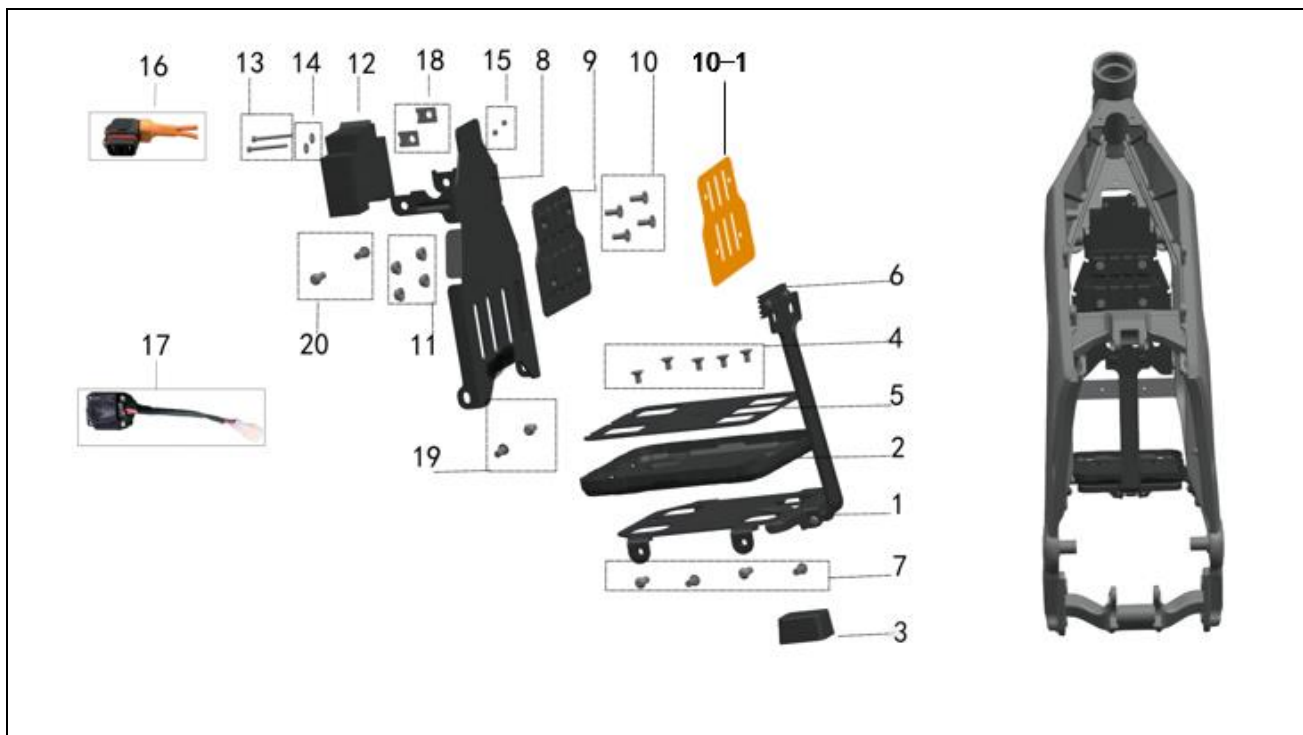
FIGURE-07 (BATTERY PACK HOLDER)
