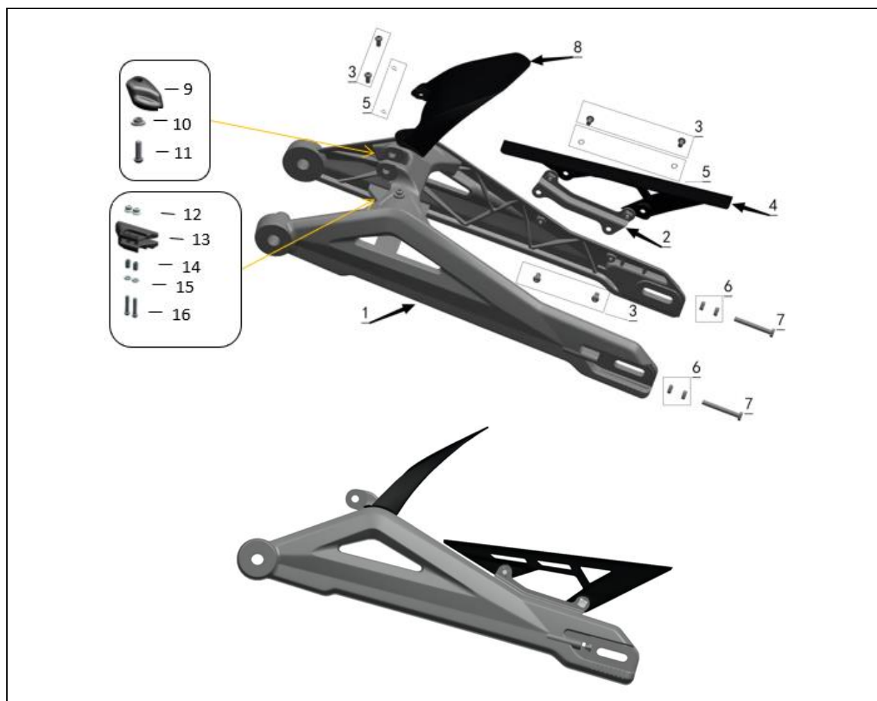
FIGURE-15 (Rr. FORK ASSY.)
