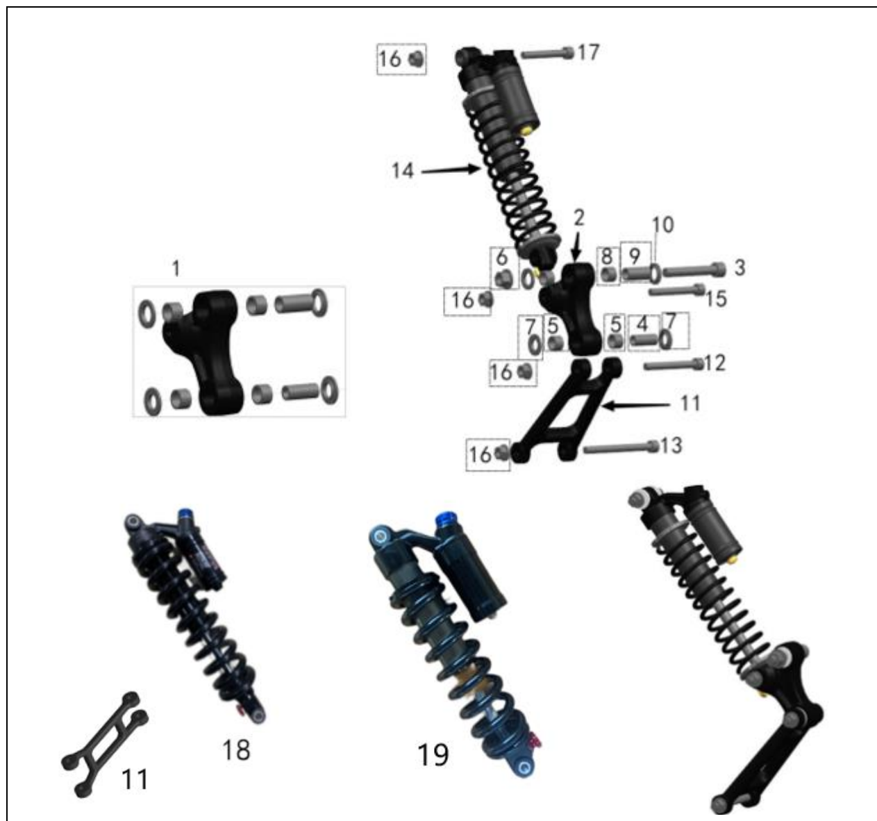
FIGURE-16 (Rr. Suspension Assy.) TALARIA
