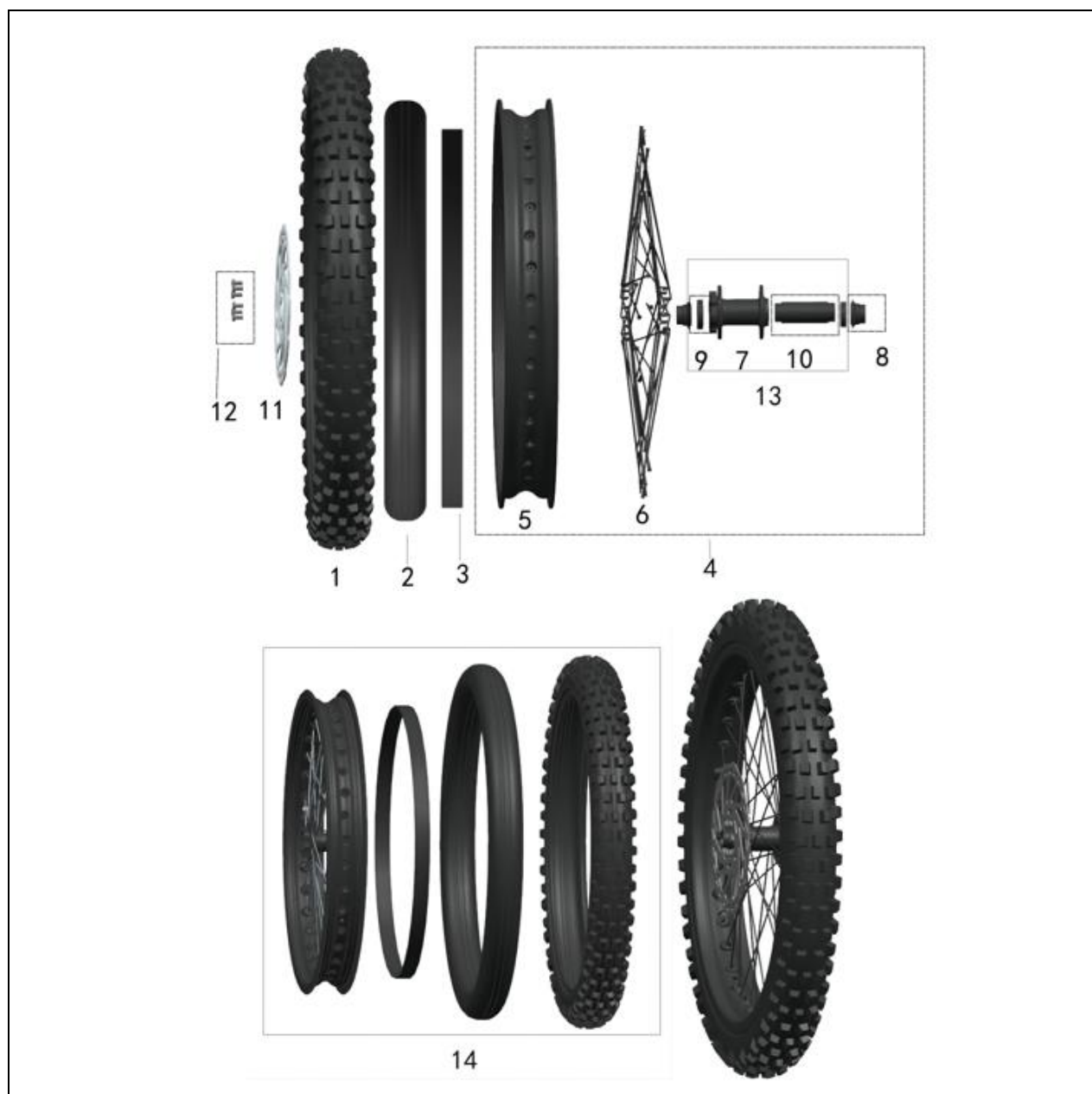
FIGURE-13 (Fr. Wheel Assy.)
