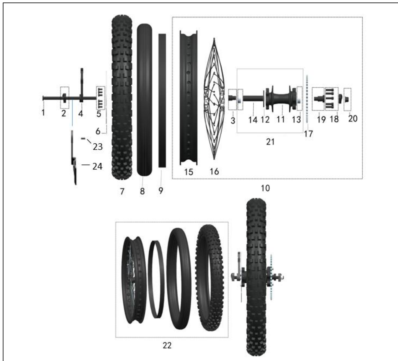
FIGURE-14 (Rr. Wheel Assy.)
