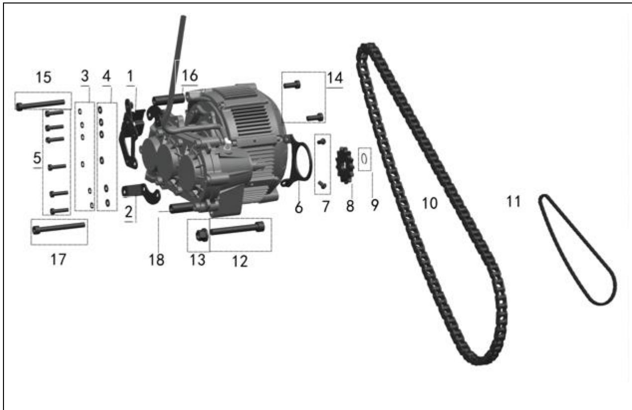
FIGURE-05 (MOTOR &amp; GEARBOX ASSY.)
