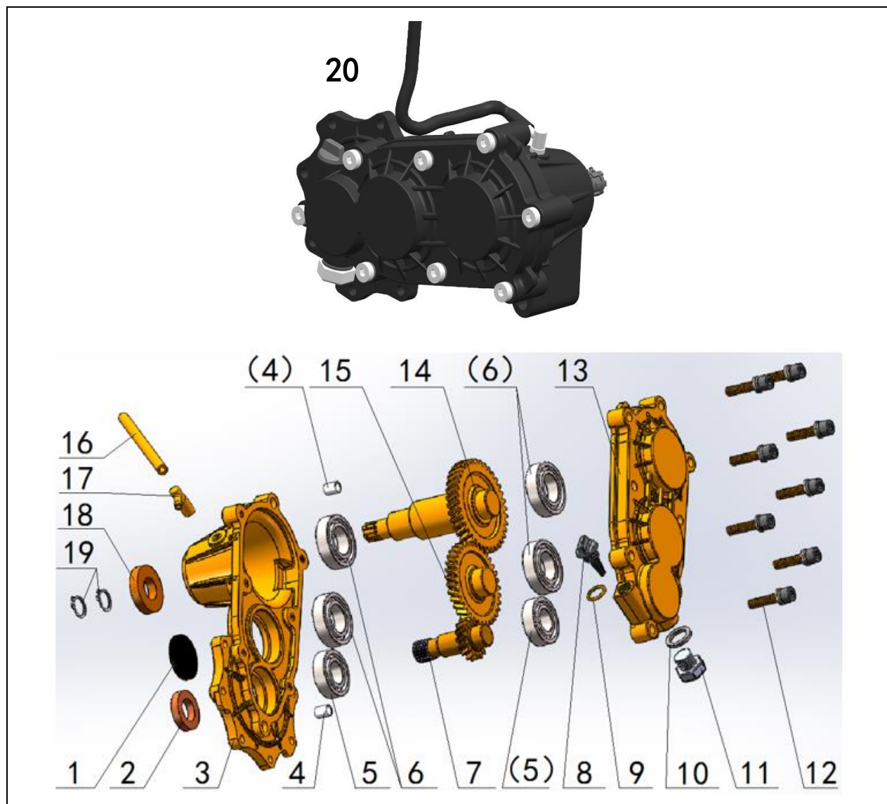
FIGURE-04 (GEARBOX ASSY.)
