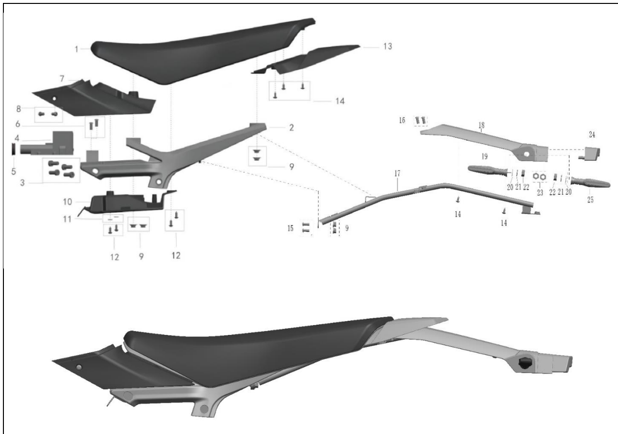
FIGURE-17 (Seat Assy.)
