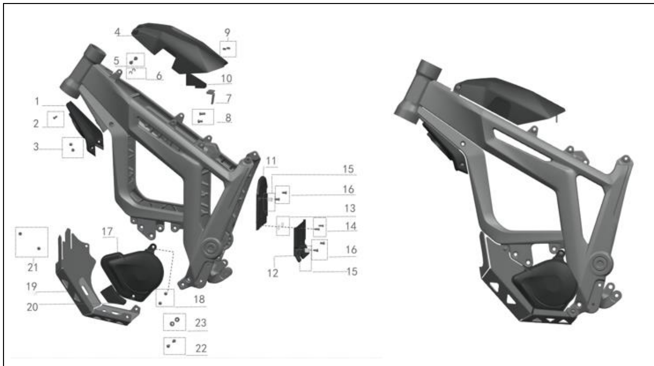
FIGURE-09 (Exterior Fixing Parts)
