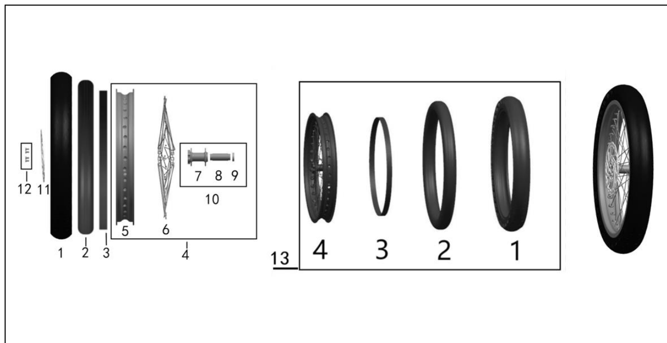
FIGURE-23-1 (Fr. Wheel Assy. - 17 inch)
