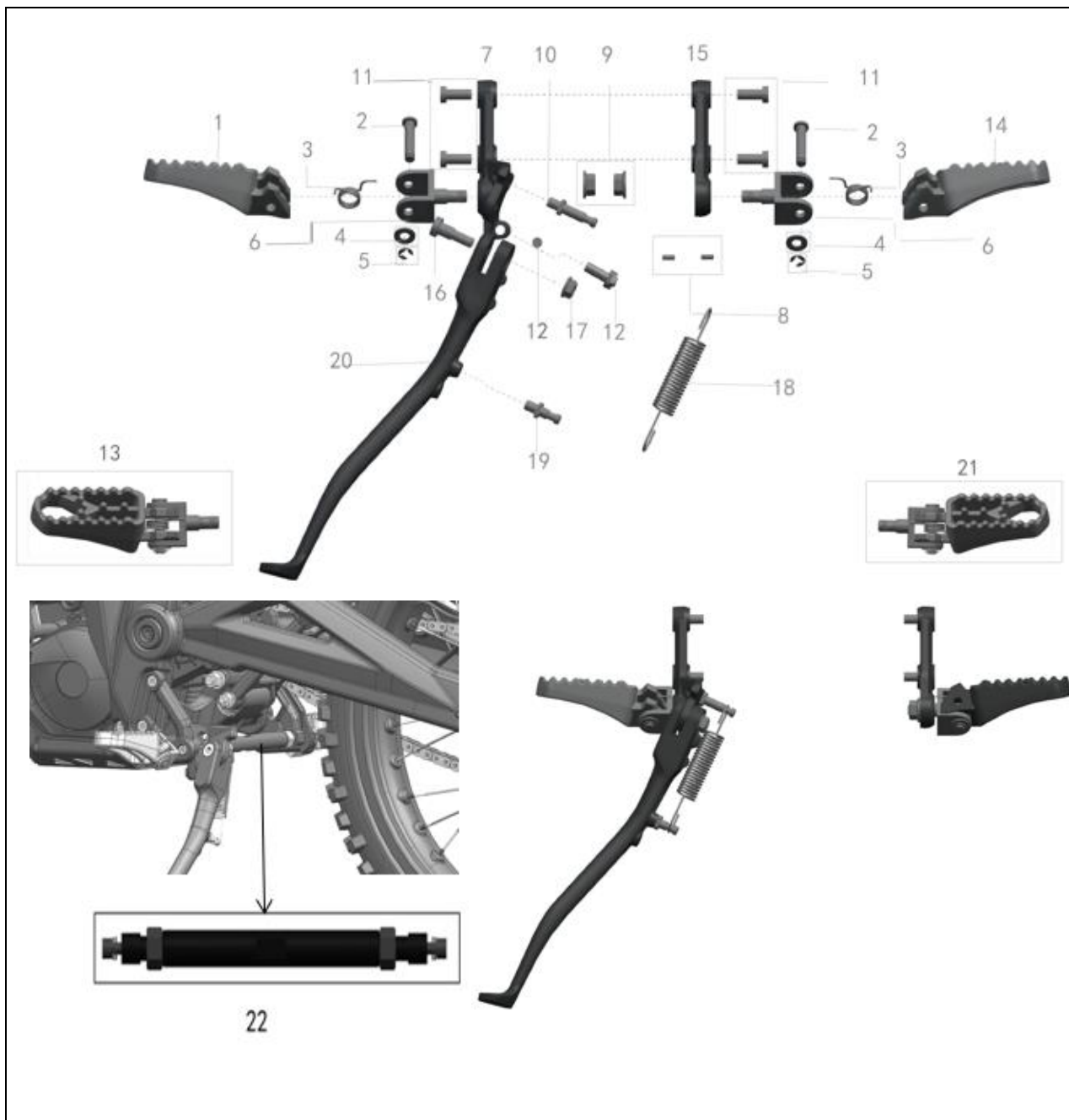
FIGURE-18 (Footpeg Assy.)
