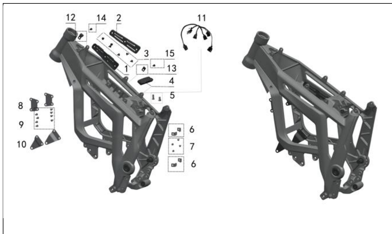
FIGURE-06(FRAME ASSY.)
