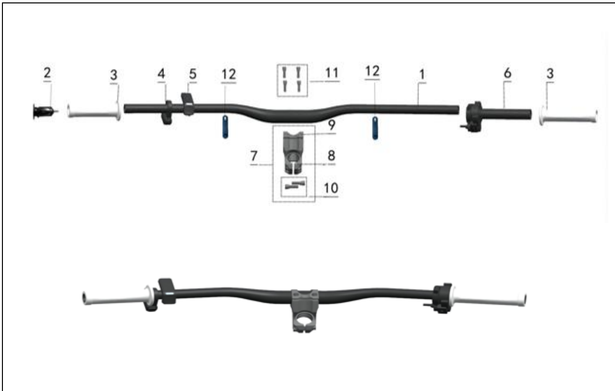
FIGURE-11 (Handlebar Assy.)
