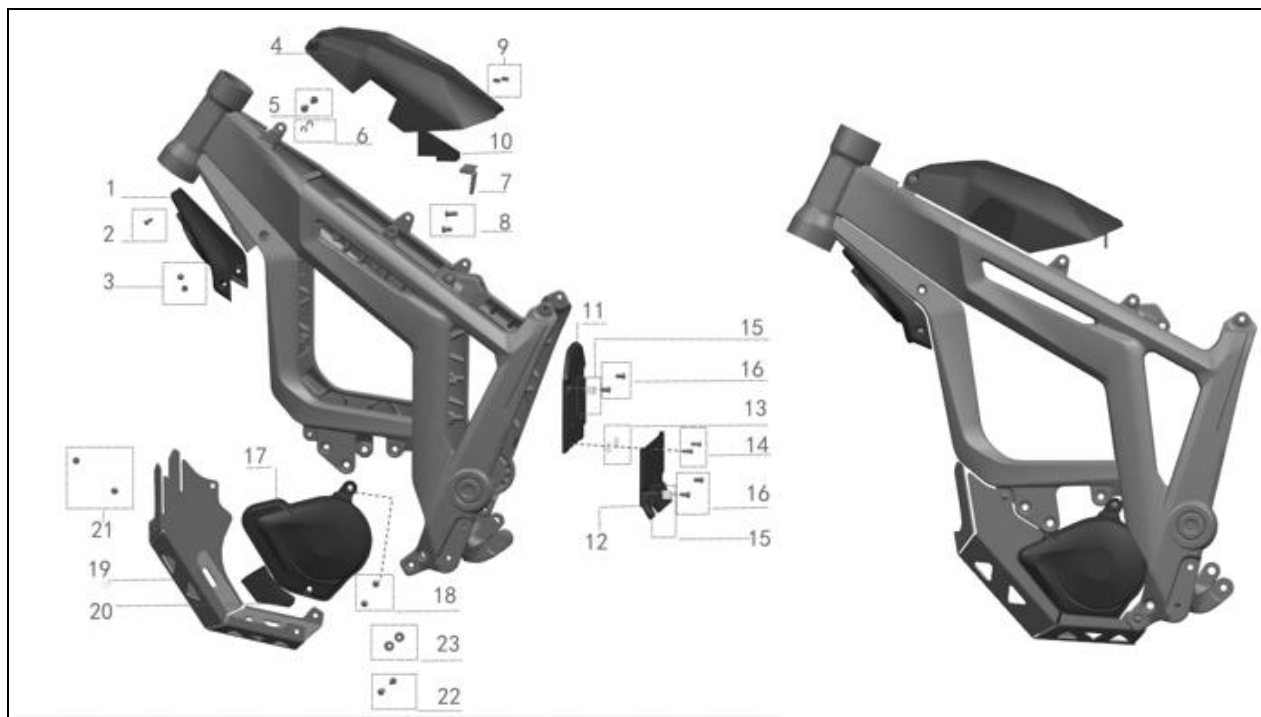
FIGURE-09 (Exterior Fixing Parts)
