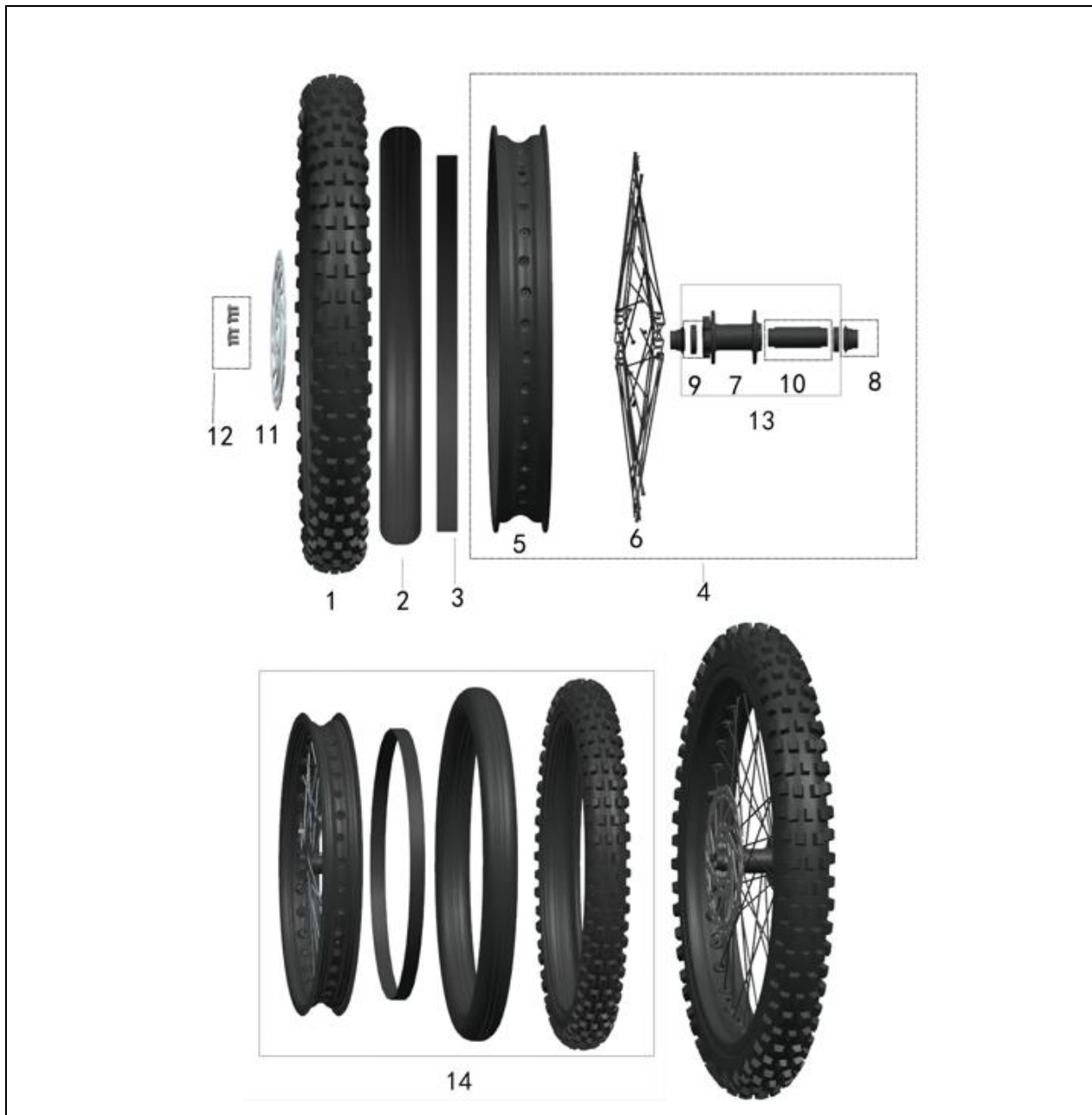
FIGURE-13 (Fr. Wheel Assy.)
