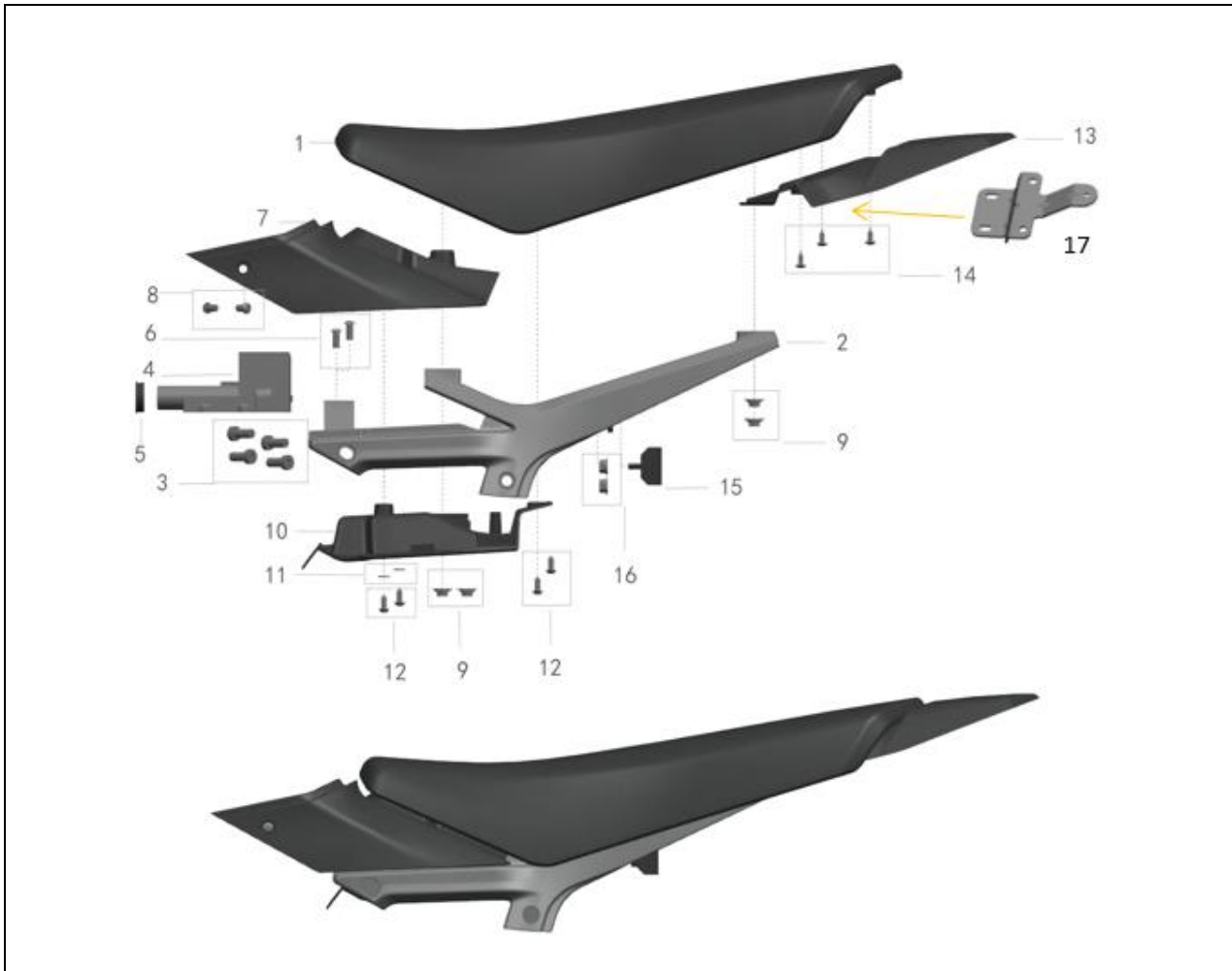
FIGURE-17 (Seat Assy.)
