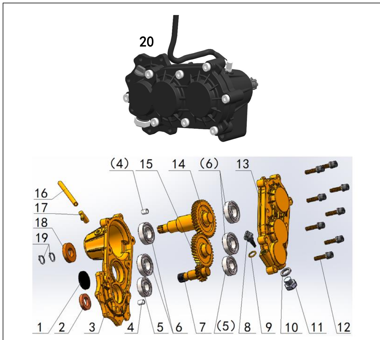
FIGURE-04 (GEARBOX ASSY.)
