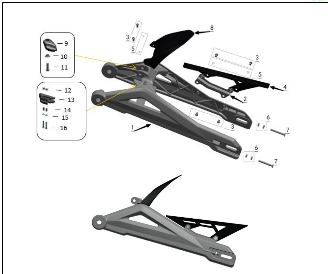
FIGURE-15 (Rr. FORK ASSY.)
