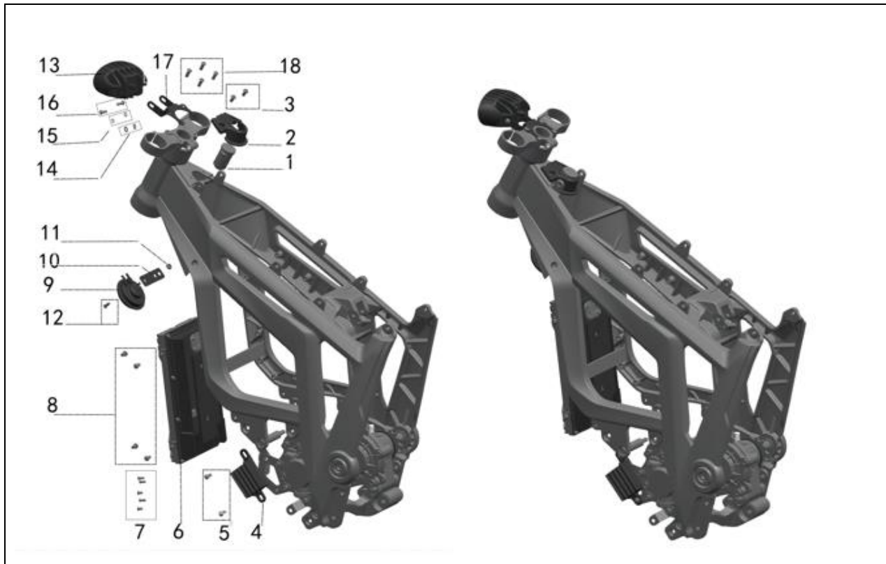
FIGURE-8 (ELECTRICAL PARTS)
